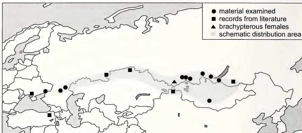
Fig. 1. Distribution area of Rhodostrophia jacularia . Literature records (black square): Vojnits 1976; Kostjuk et al. 1994; Riemis 1994; Viidalepp 1996; Hausmann 2004.
